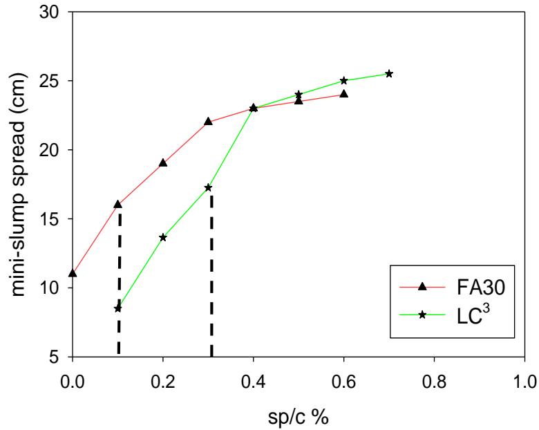
Figure 4.15 Spread curve at w/b ratio 0.45 w/b using SNF admixture
