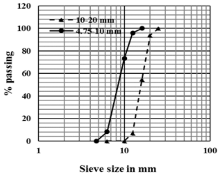
Figure 3.2 Particle size distribution of coarse aggregate (4.75-20 mm)
