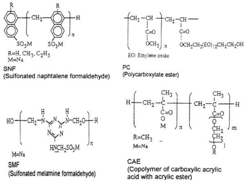
Figure 2.2 Chemical structure of different polymers in superplasticizers (Tanaka 2003; Collepari 1998; Malhotra et al., 1995; Uchikawa 1994)
