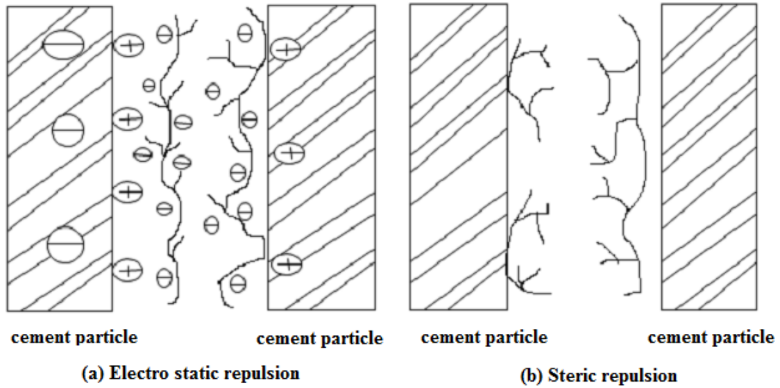
Figure 2.4 Mechanism of action of superplasticizers (Aitcin 1998)
